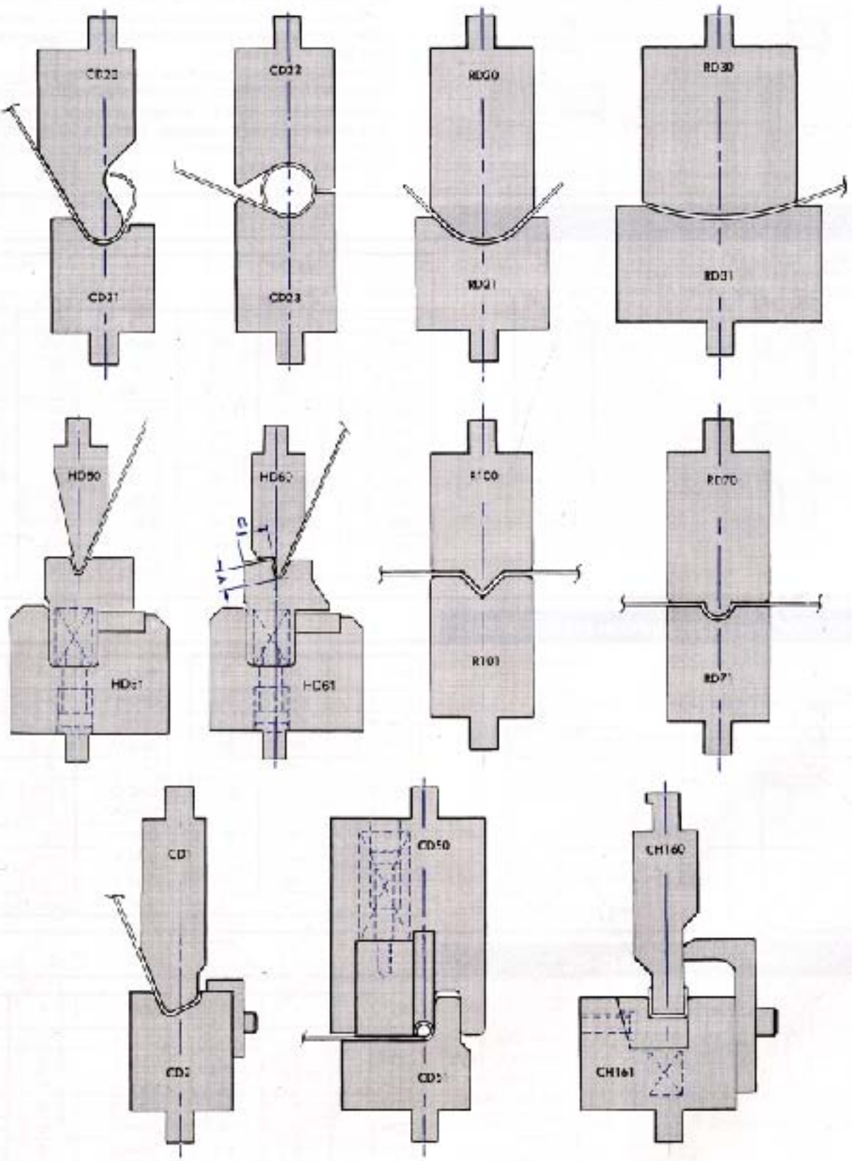
These examples of special dies show some of many types available. Consult Catalog #189 for more or send a drawing or part to our Engineering Department to evaluate your special tooling requirement.
